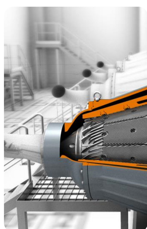
MNFC production in conical Refiner
